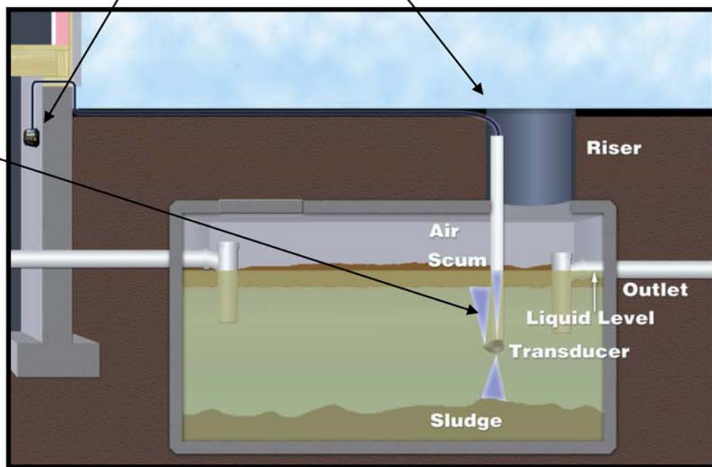
Diagram of 1000 Gallon Grease Interceptor
